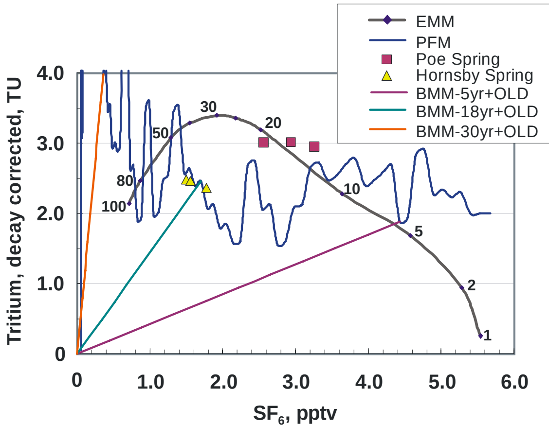
Figure 2. Comparison of \text{SF}_6 and tritium concentrations in samples of spring water to theoretical output curves for different flow scenarios using lumped parameter models including exponential mixing (EMM), piston flow (PFM), and binary mixtures (BMM) of young water (5, 18, and 30 years) with old (tracer free) water (greater than 50 years old). Ages of water along EMM curve are shown.
